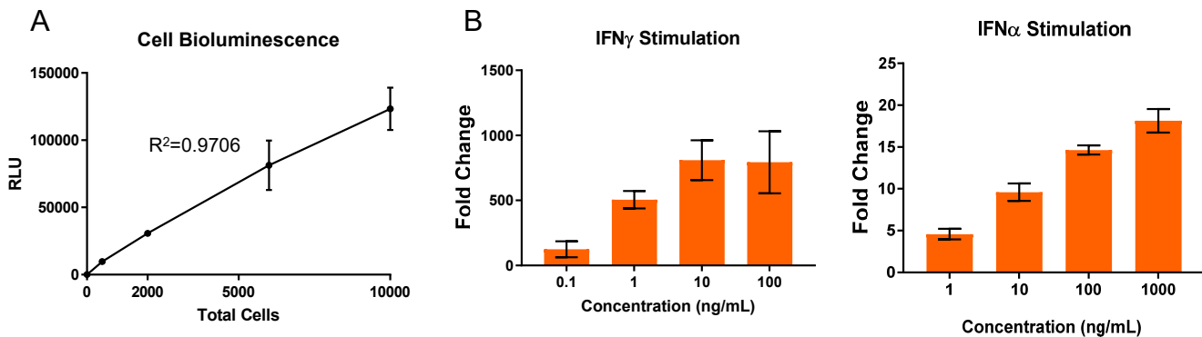
Figure 1: Linearity of luminescence and of in vitro quantification of luciferase activity of THP-1 GAS-LUC2. Cells were seeded in a 96-well plate, after stimulating overnight, bioluminescence signals were detected using Bright-glo™ (Promega®) and a luminometer (Glomax™). Error bars show standard deviation (n=3) (A) Cells were seeded at indicated cell numbers and stimulated with 10 ng/mL of IFN \gamma to determine the linear correlation of bioluminescence intensity with cell numbers. (B) Serial dilution of stimulus reagents (IFN \gamma or IFN \alpha ) to demonstrate dose response sensitivity of the GAS promoter.
